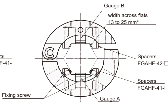
FGAH-1B-H (Hexagon shape)
