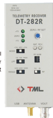
Dedicated digital telemeter receiver DT-282R
