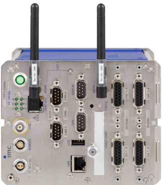
CRFX-2000G Base Unit with additional WiFi extension and DI8-DO8-ENC4-DAC4
