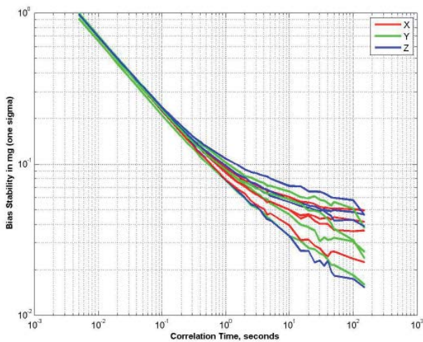
Figure 5.15 Accelerometer Stability
