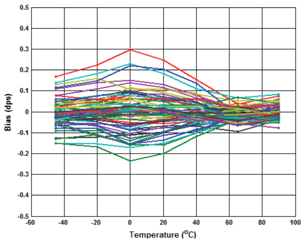
Figure 5.1 Gyroscope Bias
