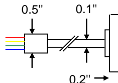
Option code 5 - End exit integral MI (mineral insulated) stainless steel cable
